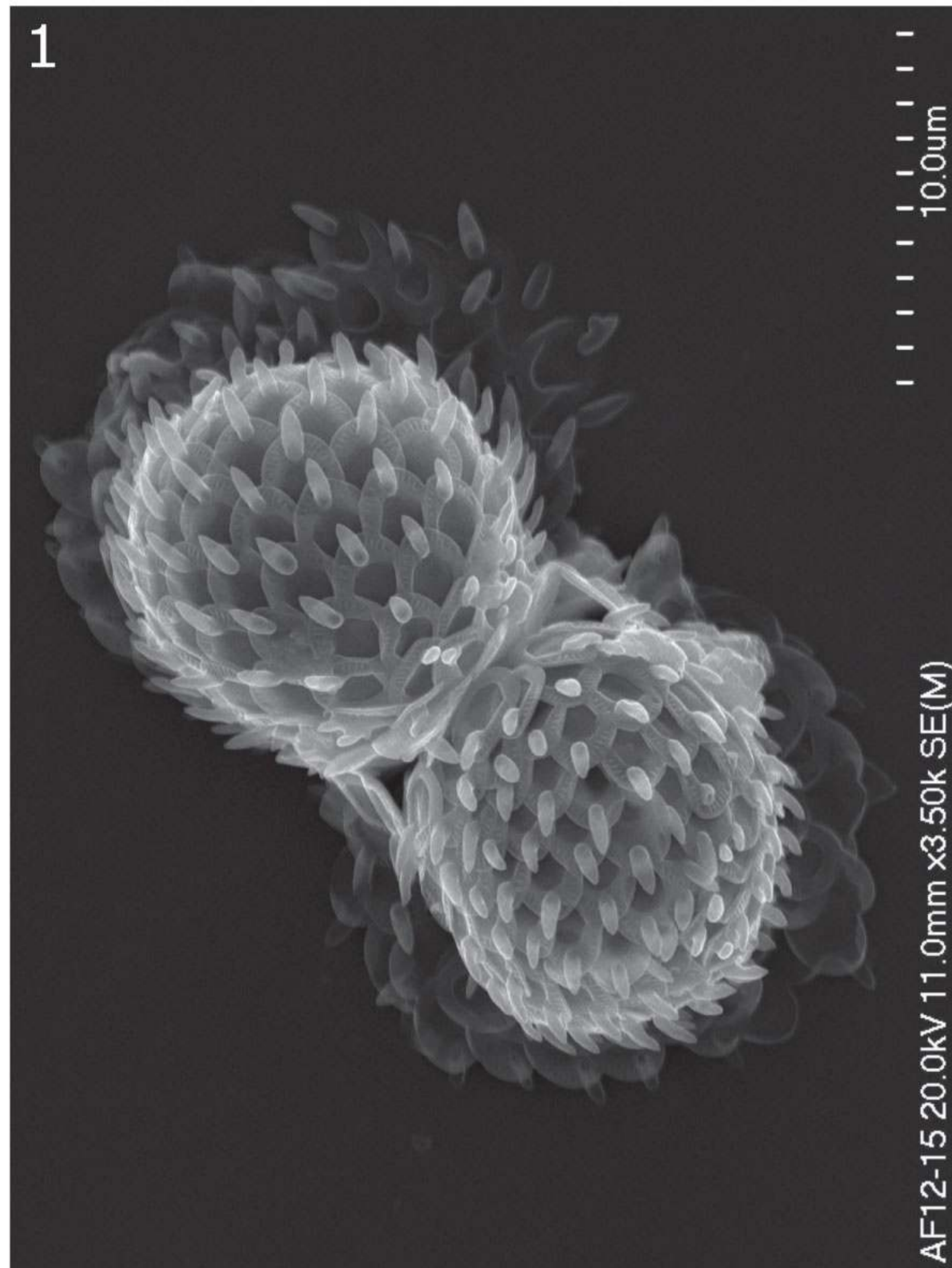
Synura echinulata Koršikov, 1 – two cells with well visible connection, 2 – one cell in higher magnification with well visible arrangement of scales, 3 – ultrastructure of scales.
