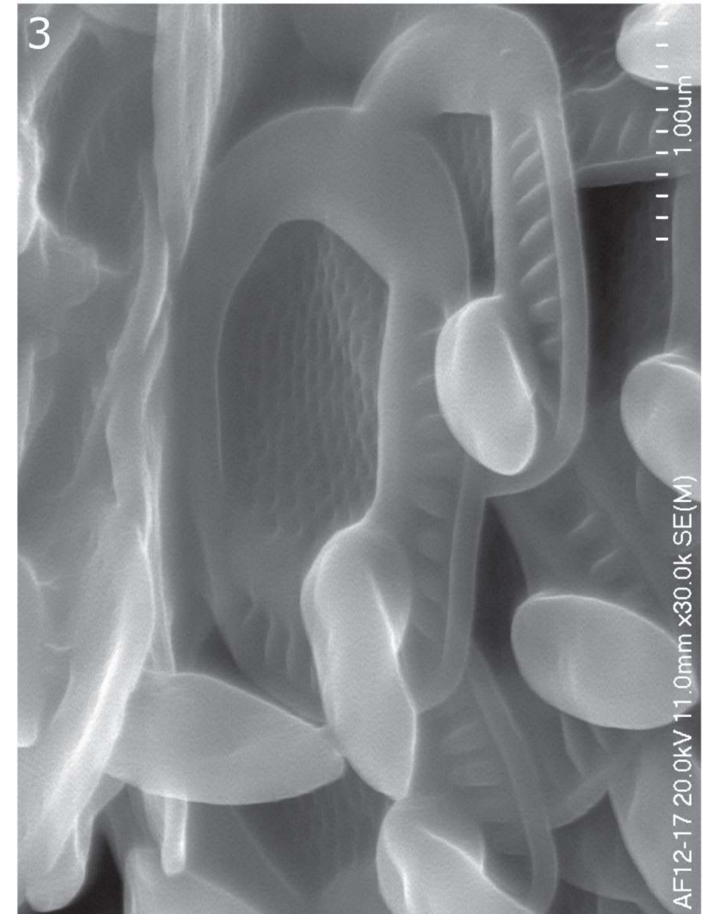
Synura echinulata Koršikov, 1 – two cells with well visible connection, 2 – one cell in higher magnification with well visible arrangement of scales, 3 – ultrastructure of scales.
